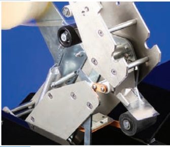
Top and bottom tape heads are interchangeable and tip back for easy threading.
